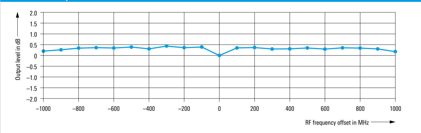
Measured frequency response of the R&S®SMW200A/R&S®SZU100A combo at 60.48 GHz carrier frequency and +0 dBm output level
